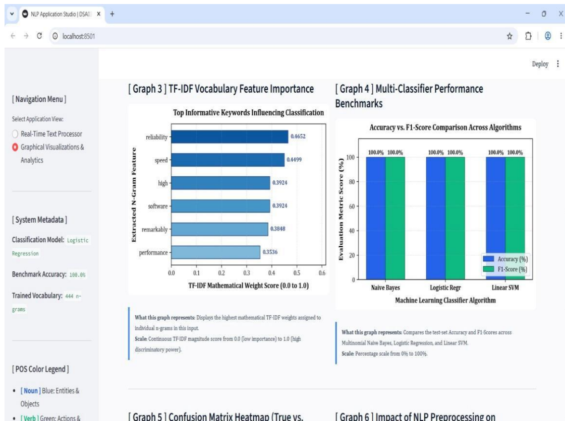
Fig 3.3 – TF-IDF feature importance and multi-classifier performance benchmarks
